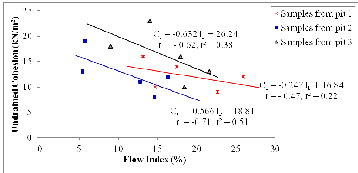
Figure 4: Regression plots of cohesion and flow index of the studied soils
