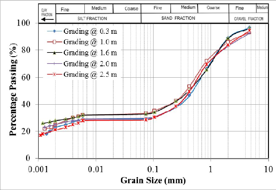
Figure 3c: Grain-size distribution curves for soils from Pit 3
