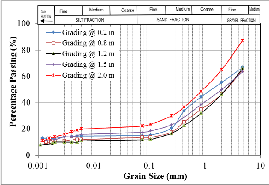
Figure 3b: Grain-size distribution curves for soils from Pit 2
