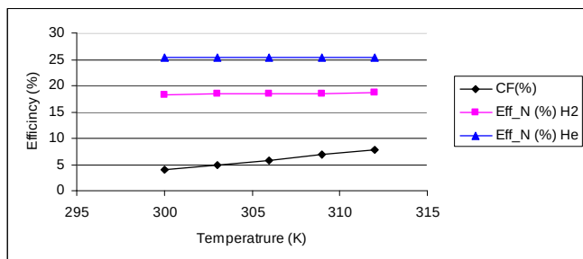
Fig. 6. The performance results showing of the net efficiency with respect to the amount of available heat rejected by the condenser versus the top cycle temperatures with the data shown in table 5.
