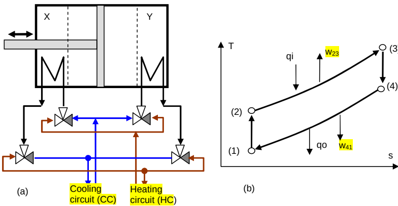
Fig. 4. The processes of heating and cooling a fluid at constant pressure undergoing closed transformations: (a), the non regenerative engine structure showing the heat exchangers actuating alternatively as heater and cooler, (b), the corresponding non regenerative T-s diagram.
