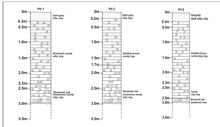
Figure 2: Test pit and soil profiles from the study area
