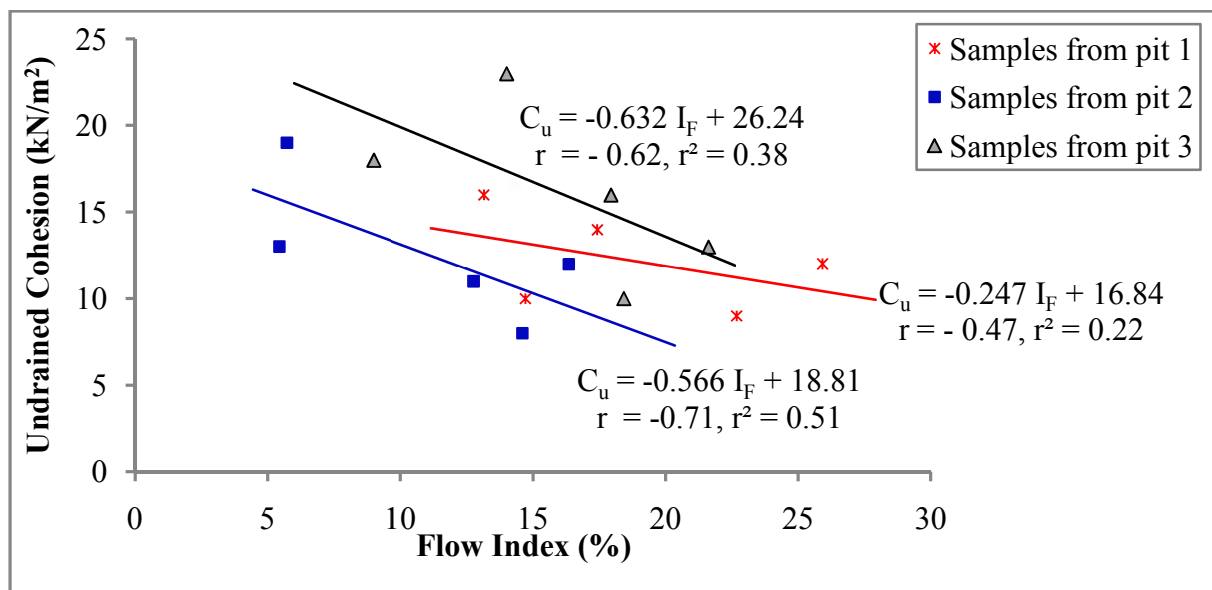
Figure 4: Regression plots of cohesion and flow index of the studied soils
