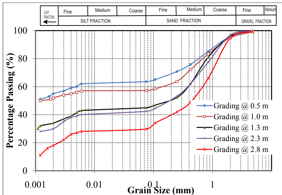
Figure 3: Grain-size distribution curves for soils from Pit 1
