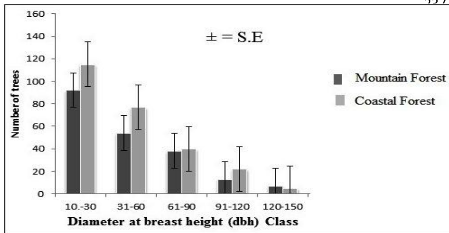
Figure 3. Diameter class of trees destroyed in the Montane and coastal forest
