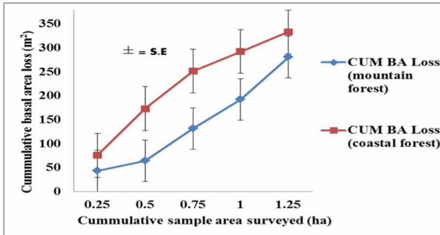
Figure 2: Cumulative basal area loss in the coastal and montane forest in the study sites
