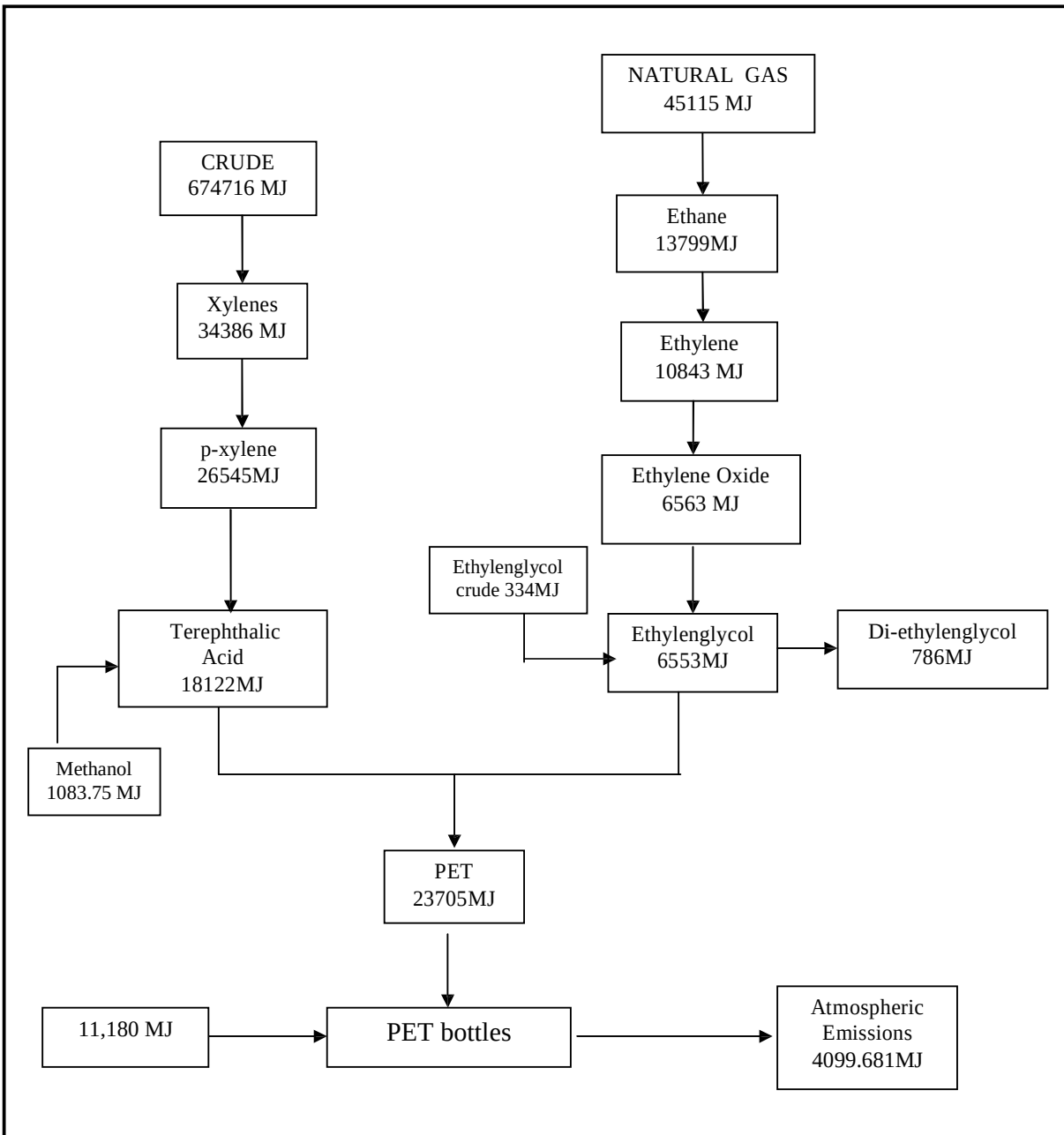
Figure 3. Flow diagram to produce PET bottles and Exergy balance of production.
