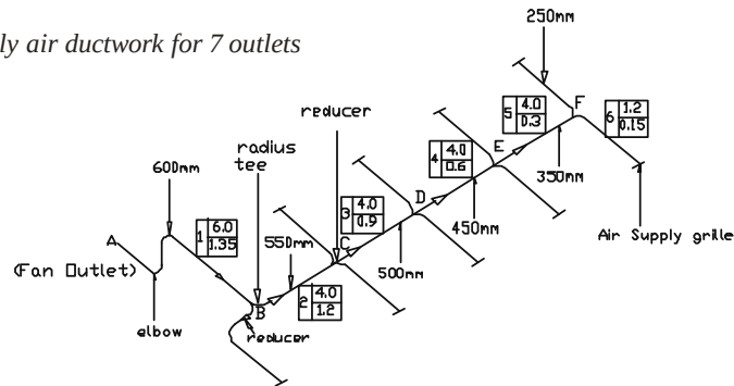
Fig. 6: Isometric sketch of supply air ductwork for 9 outlets
