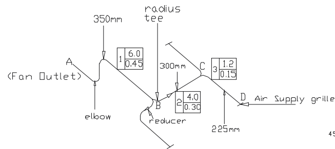
Fig. 3: Isometric sketch of supply air ductwork for 3 outlets
