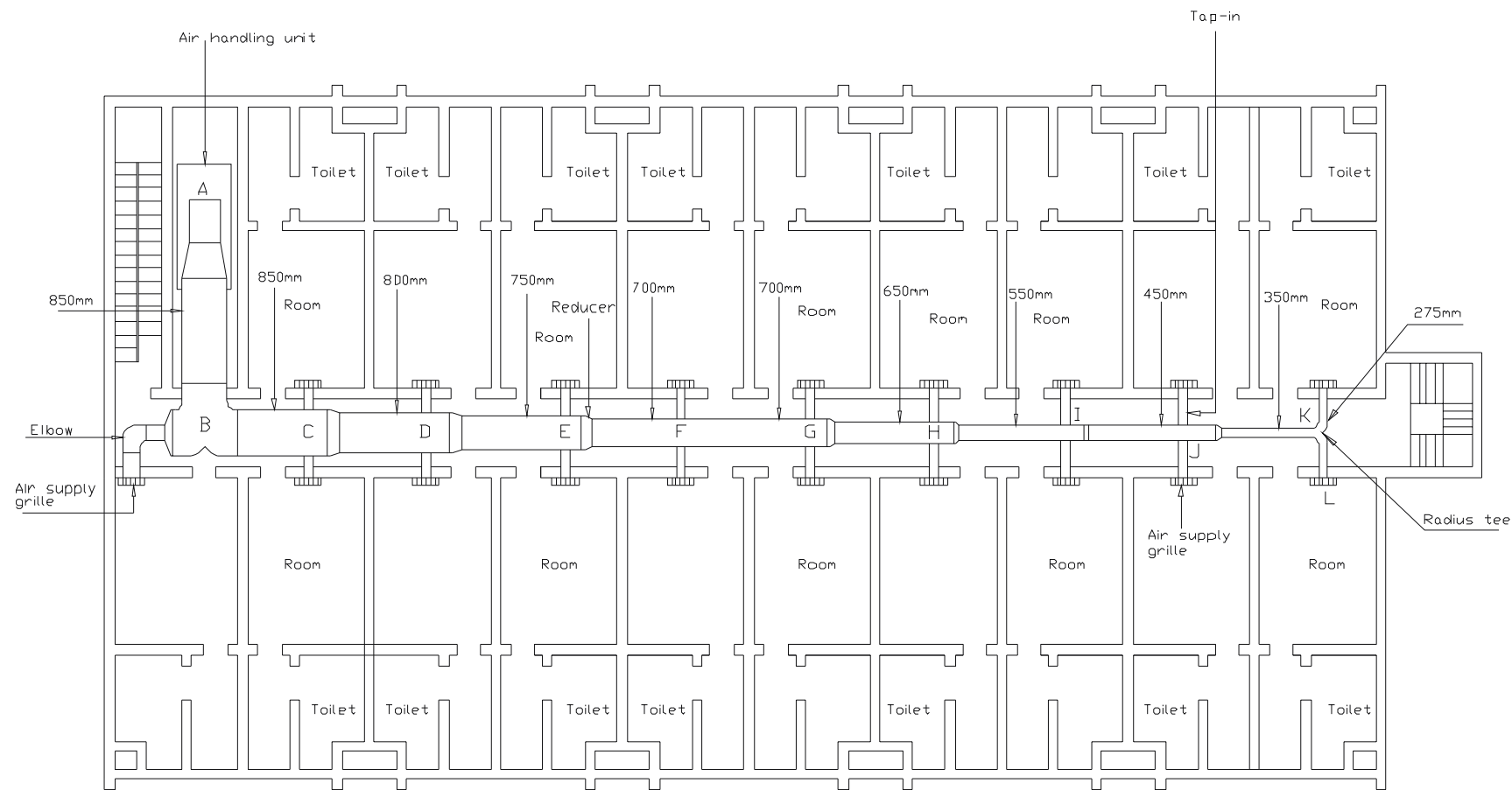
Fig. 1: Plan of air distribution ductwork
