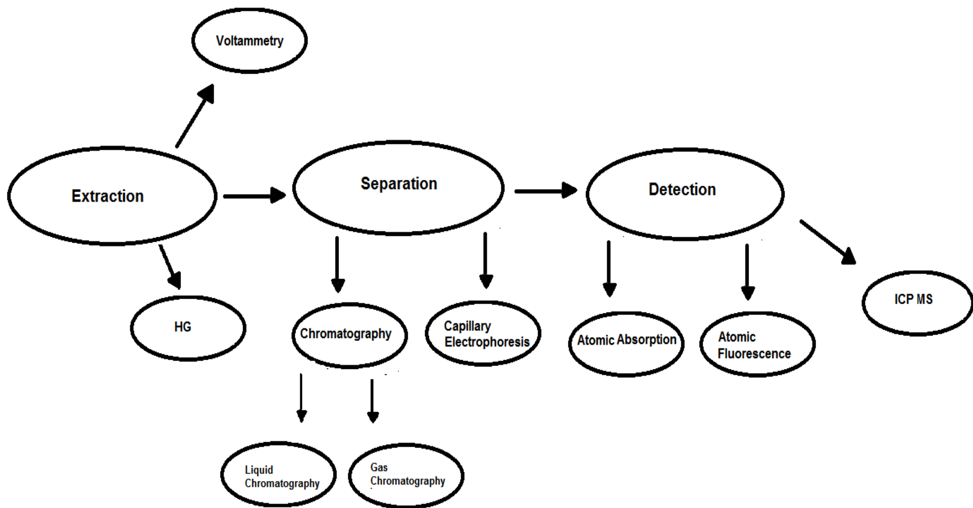
Figure 1. Techniques involved in arsenic speciation analysis
